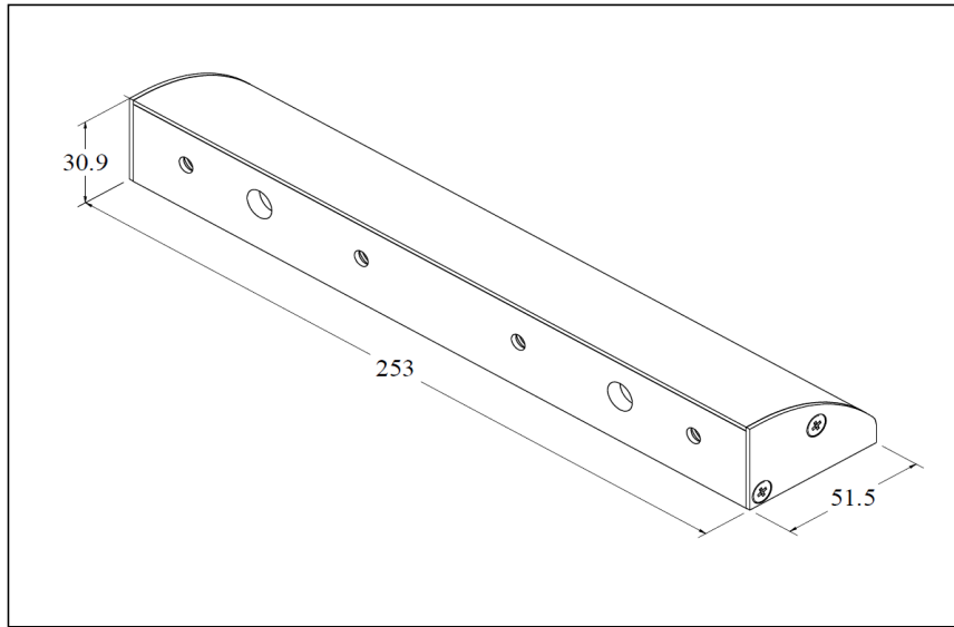
600 LBS EM LOCK LSDC-275-G BRACKET Dimension : 253mm (L) X 51.5mm(W) X 30.9mm(H)
